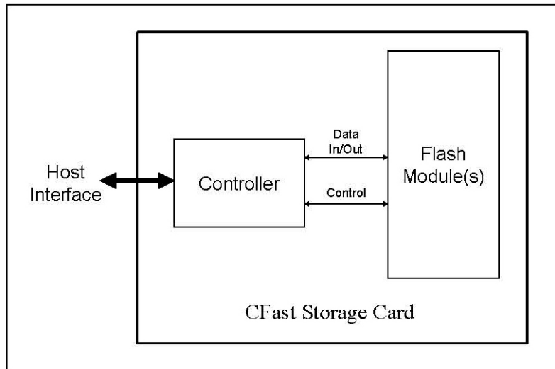
Figure 1: CFast Storage Card Block Diagram
