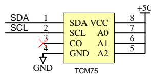
Figure 4-2: Digital Temperature Sensor
