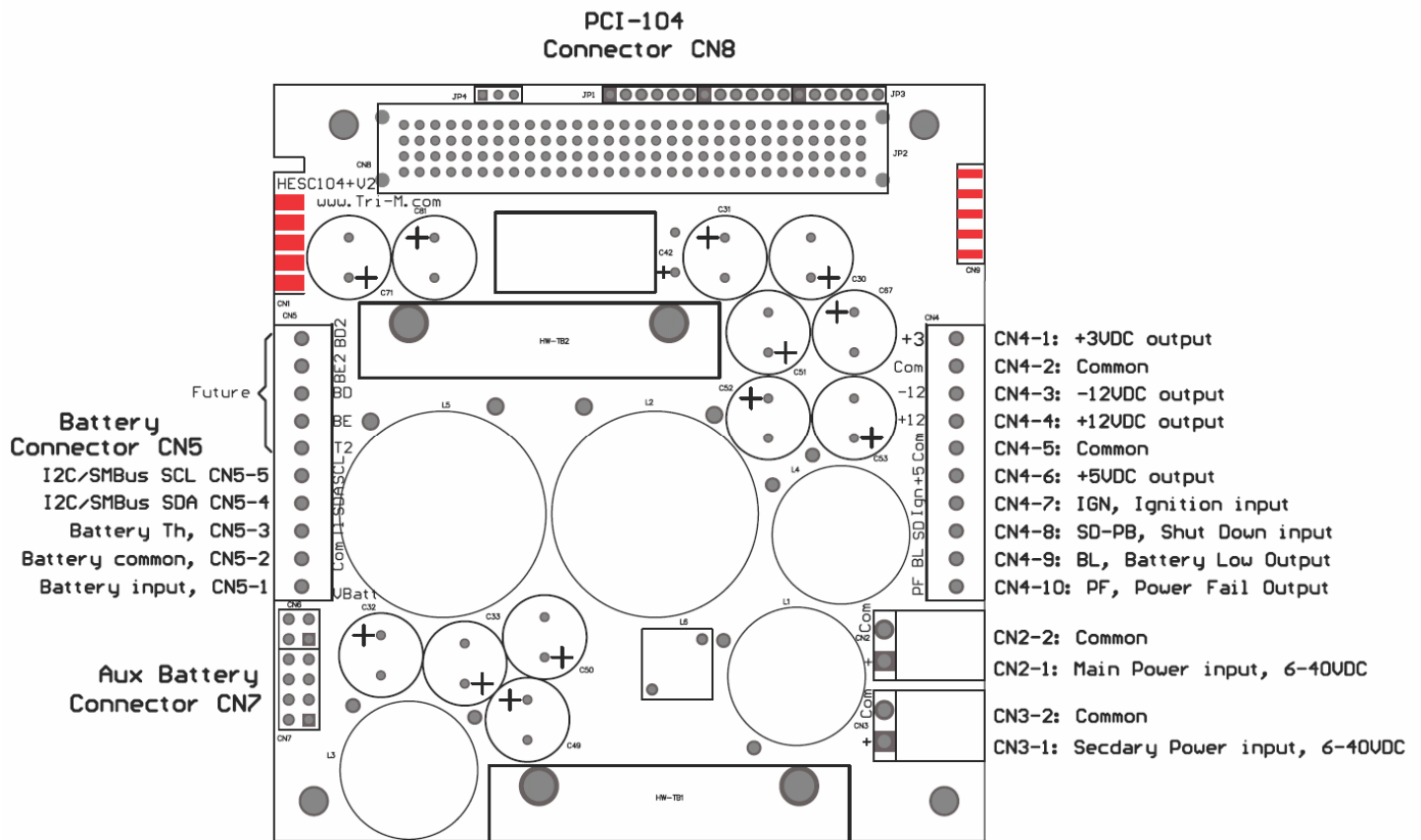
Figure 2-1: HESC104+ Connectors
