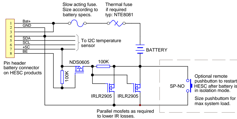
Figure 4-1: Battery Mosfet Isolation Circuit
