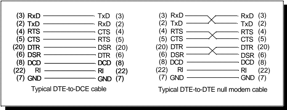
Figure 14 --- Cabling requirements for RS-232-C devices (cables using 25-pin connectors shown)
