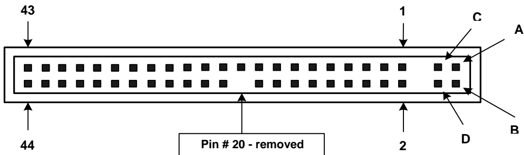
Figure 3 Pin Location
