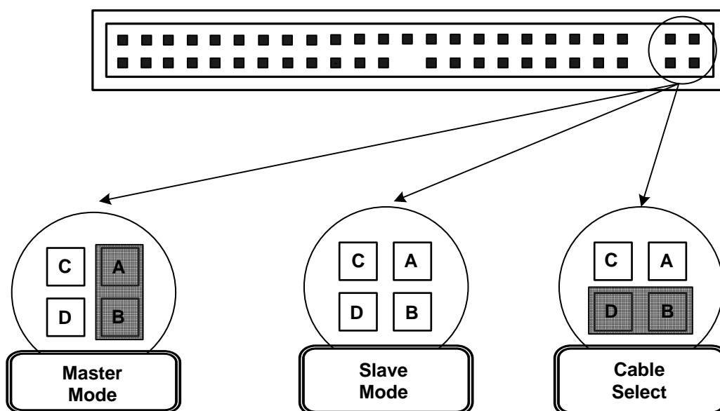
Figure 4 Jumper Settings
