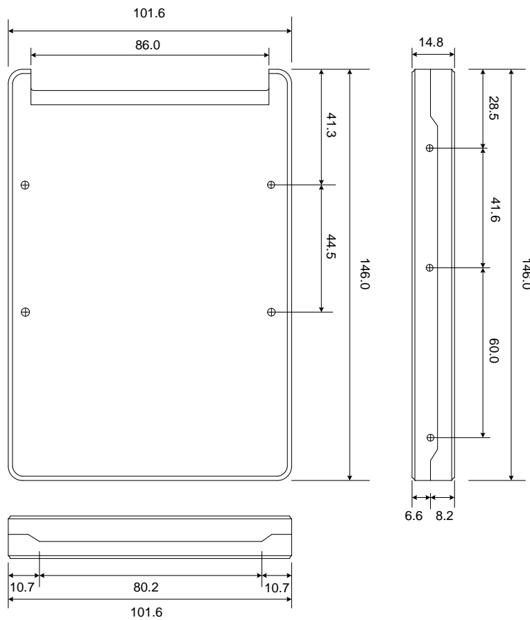
Figure 2 Physical Dimensions
